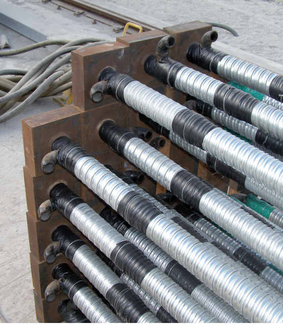
Prefabricated bar tendons
